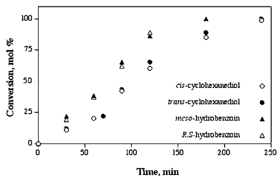
Figure 2. Kinetic profile of the oxidation of stereoisomers of 1,2-cyclohexanediol and 1,2-diphenyl-1,2-ethanediol. Reaction conditions: 250 mM diol, 10 mM \text{Q}_3\text{H}_2[\text{IMo}_6\text{O}_{24}] in acetonitrile at 80^\circ\text{C} under 2 atm oxygen.
