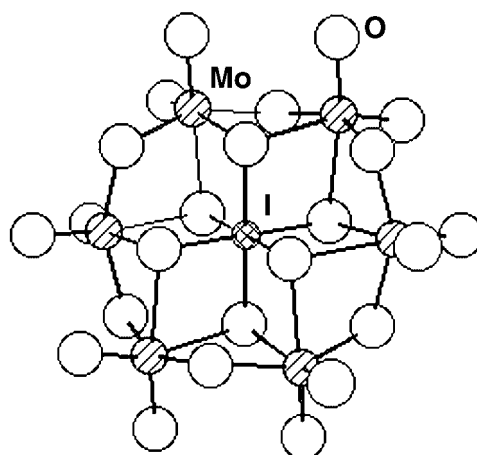
Figure 1. The Anderson-type [\text{I}^{\text{VI}}\text{Mo}_6\text{O}_{24}]^{5-} polyoxometalate.
